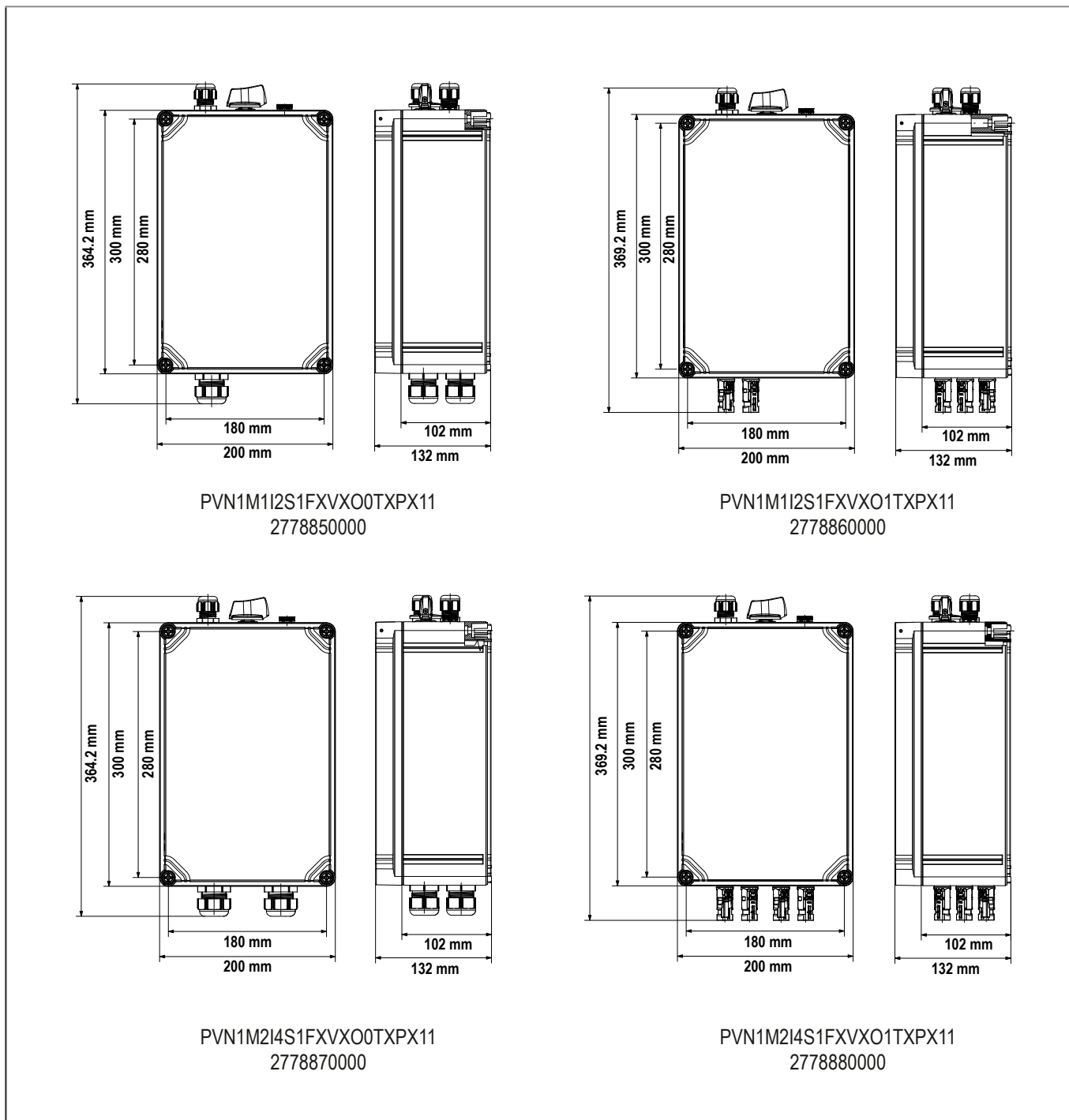
Figure 5.5 Dimensions for direct mounting without mounting brackets
