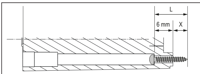
Figure 5.4 Drill hole depth for wall mounting
