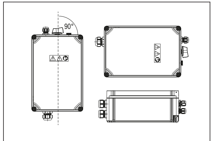
Figure 5.1 Vertical and horizontal alignment and mounted horizontally lying on the back
