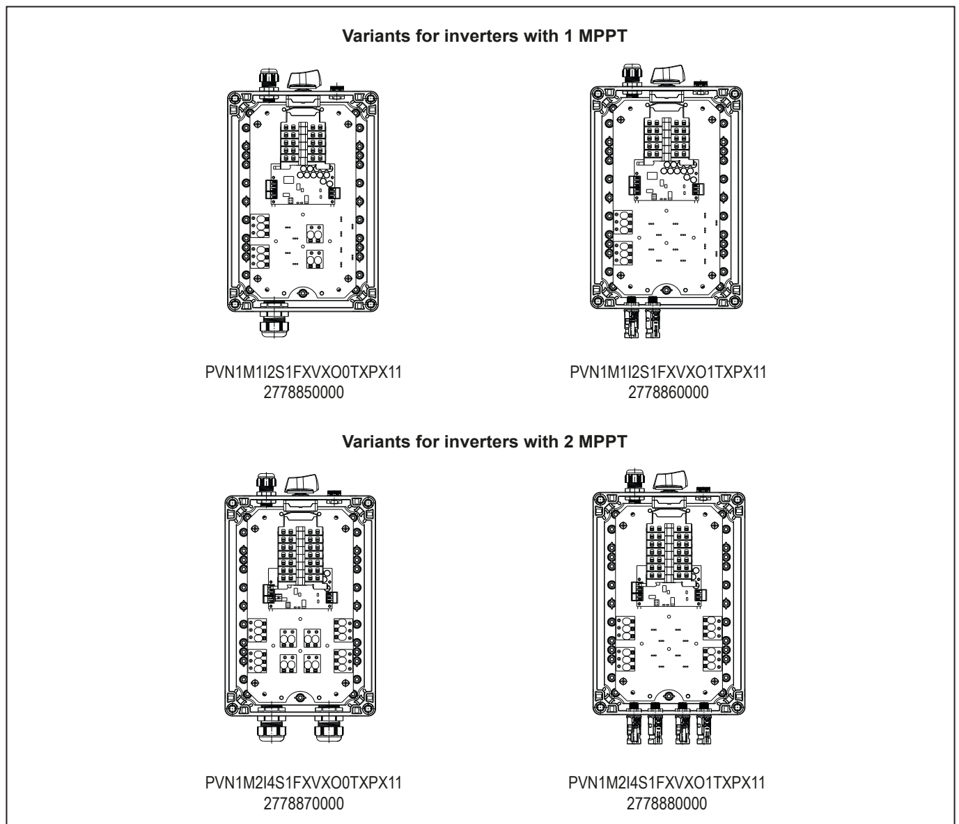
Figure 3.1 Overview of product variants
