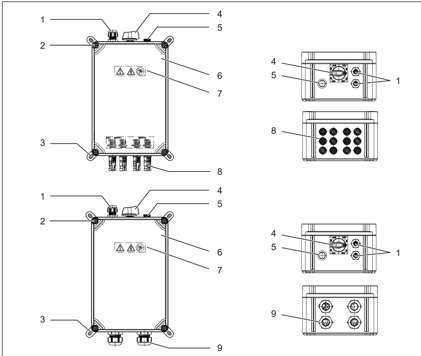
Figure 3.2 Product overview (example)
