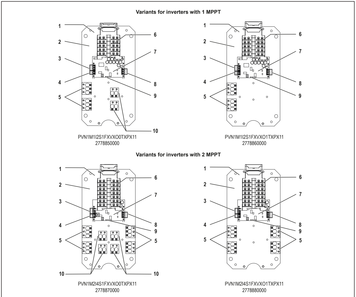
Figure 3.3 Overview of components on the PCB
