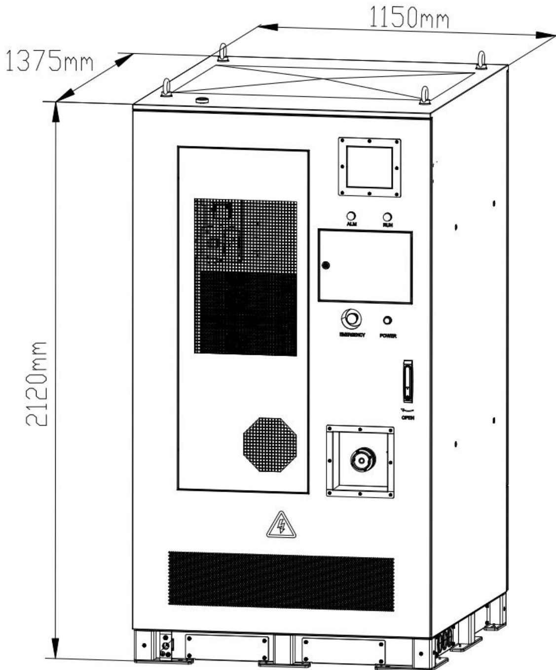
Figure 3.1.4.1 Schematic of Cabinet Dimension
