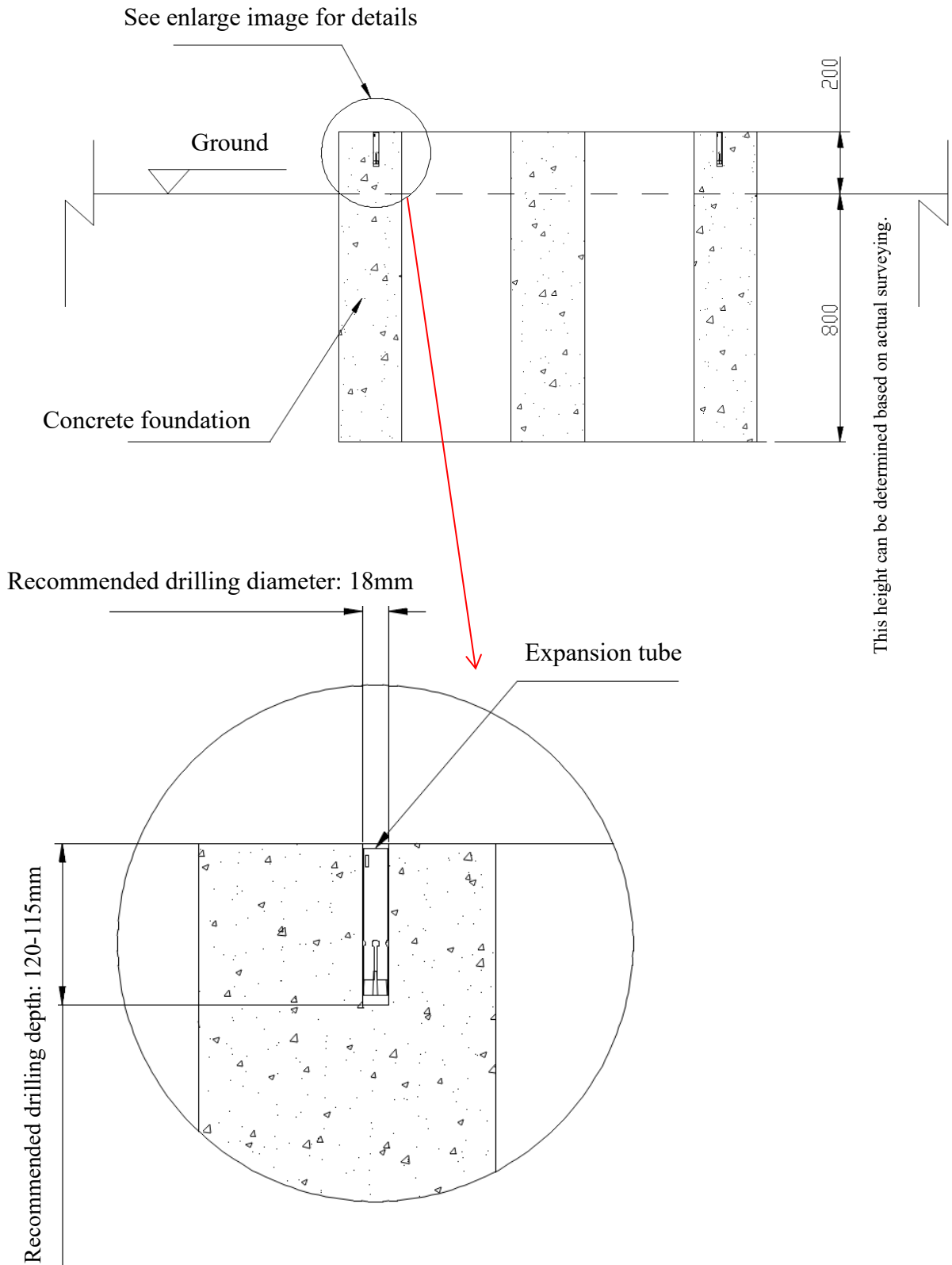
Figure 5.2.2.3 Diagram showing the pre-buried expansion tube
