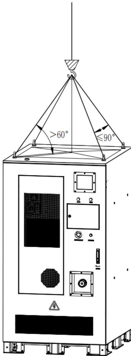
Figure 5.2.3.1 Lifting Schematic
