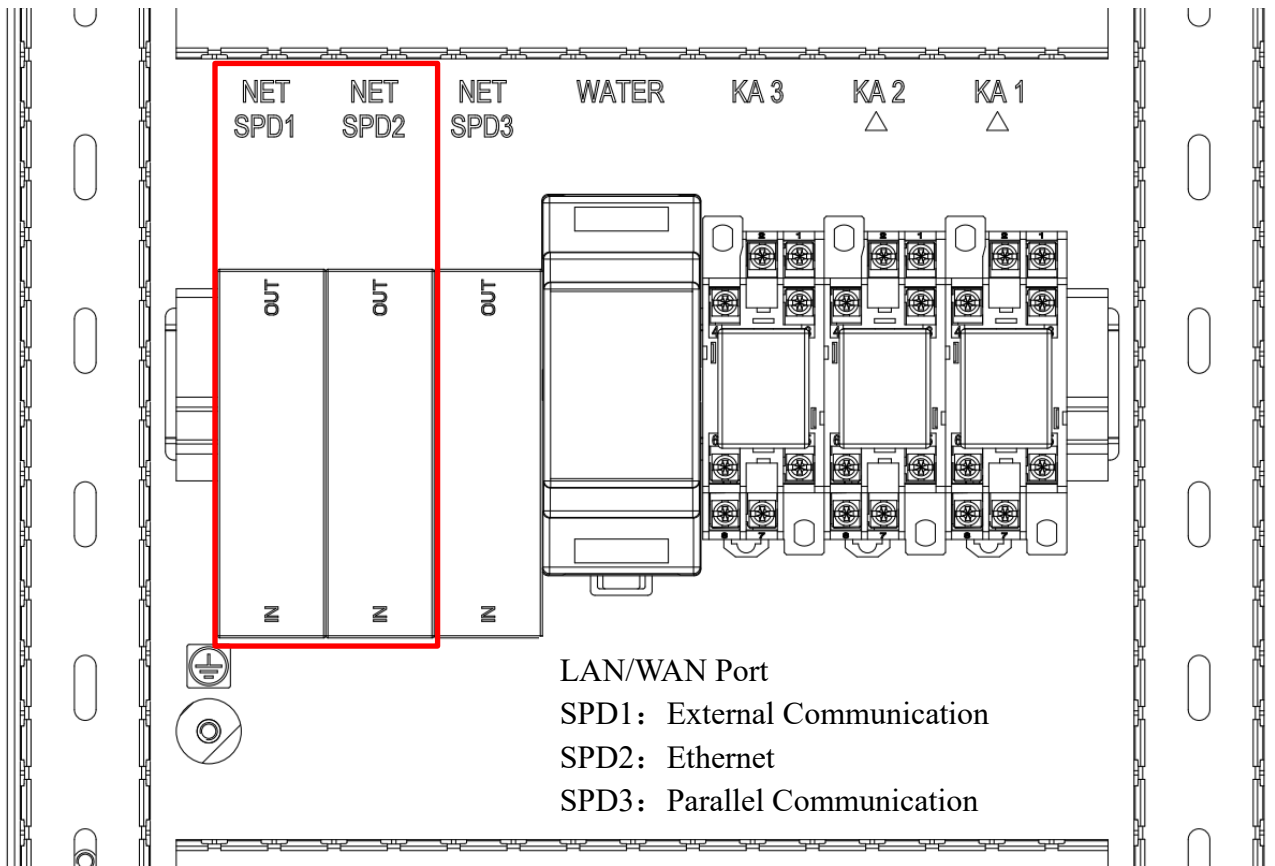
Figure 5.3.5.1 Communication Wiring Location Diagram
