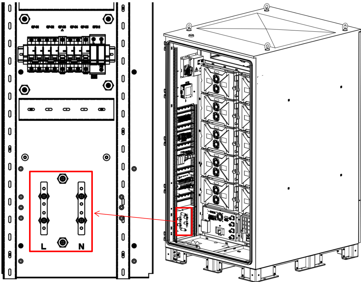
Figure 5.3.4.2 Schematic Diagram of Auxiliary Power Cable Connection Locations
