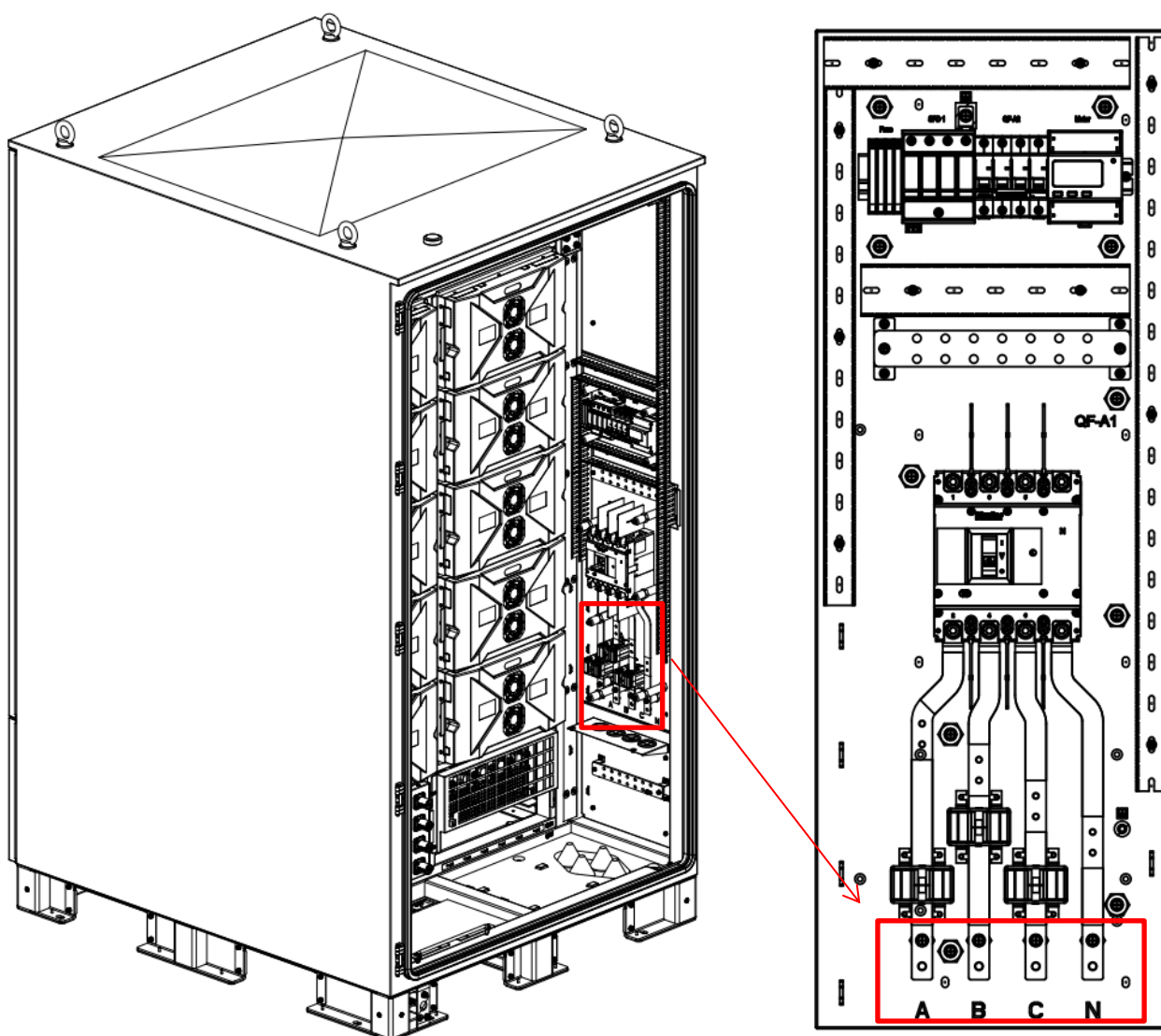
Figure 5.3.4.1 Schematic Diagram of Power Cable Connection Locations
