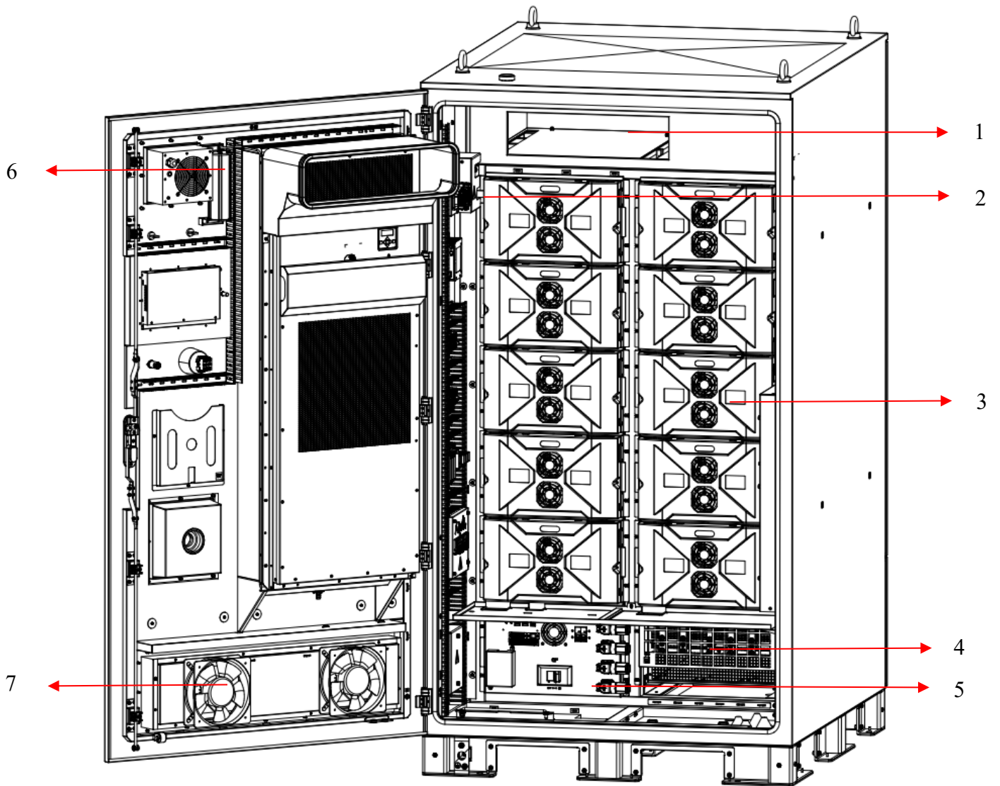
Internal Layout Diagram
