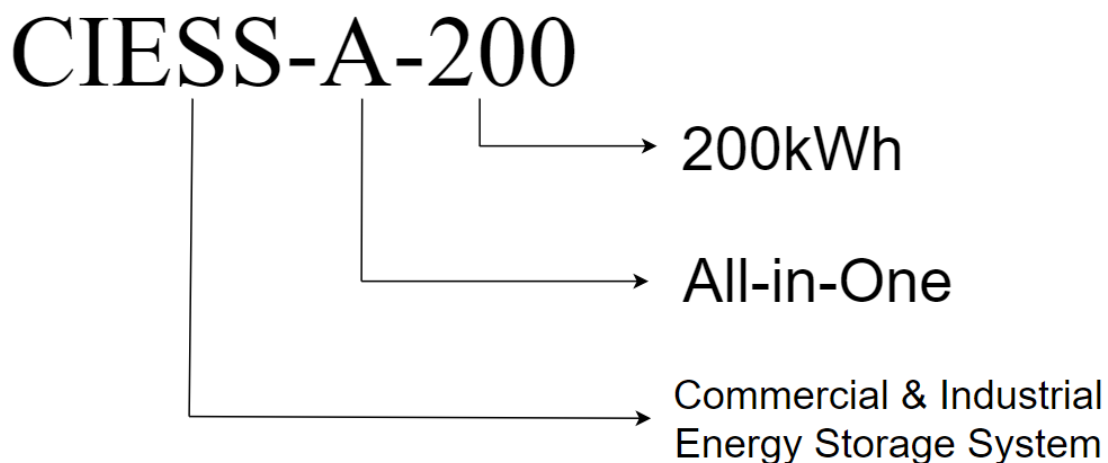
Figure 1.2.1 Description of model
