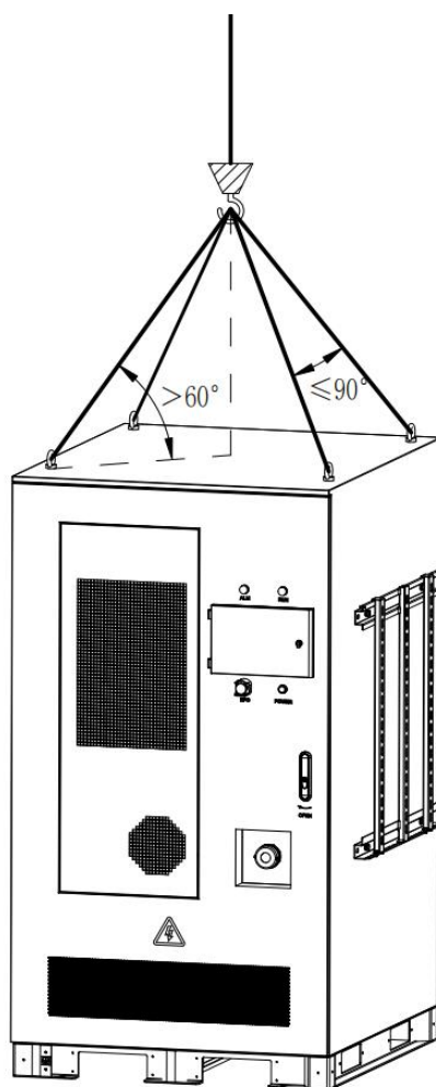
Figure 5.2.3.1 Lifting Schematic
