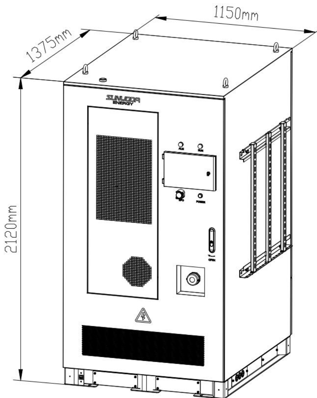
Figure 3.4.1 Schematic of Cabinet Dimensions
