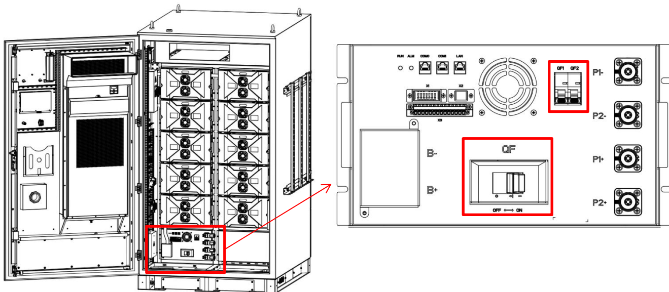
Figure 6.2.2.2 Schematic diagram of the control box
