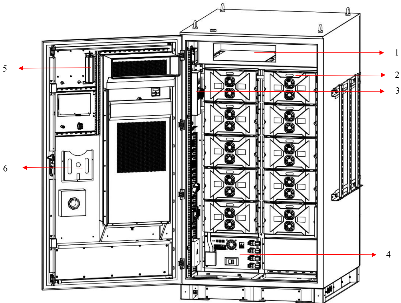
Internal Layout Diagram
