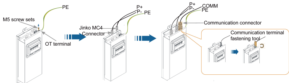
Connection Diagram
