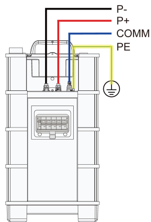
Connection Diagram
