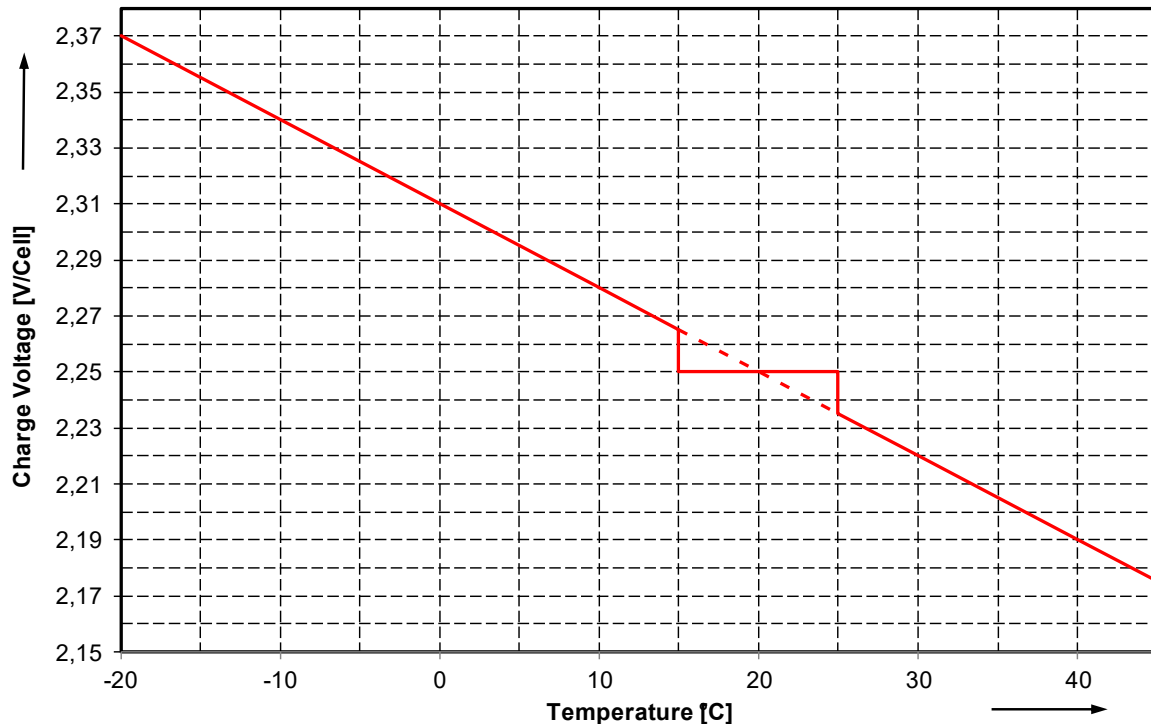
Figure 7.2.2-1 - Temperature-dependent adjustment of the float charge voltage for battery types with a float charge voltage of 2.25 V/cell at T_{nenn}
