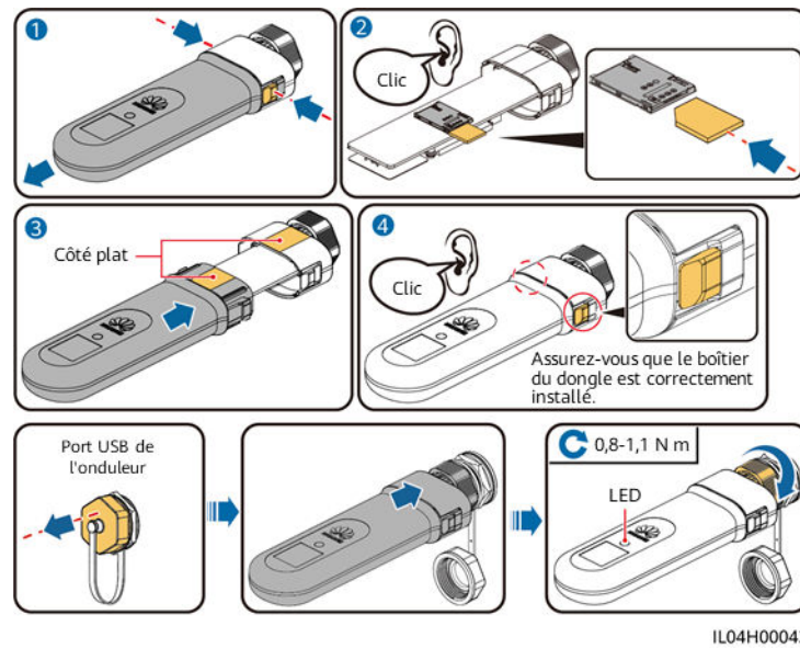
Figure 5-45 Installation d'un dongle intelligent 4G (SDongleB-06)
