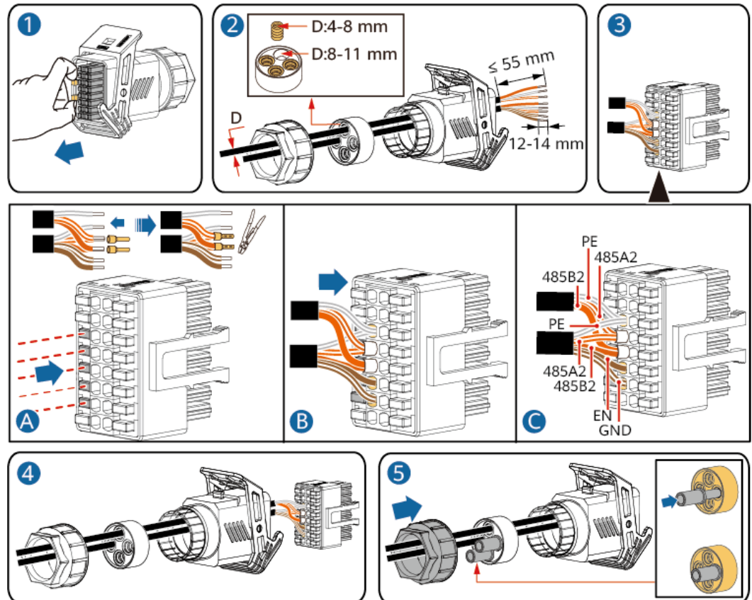
Figure 5-32 Installation du câble
