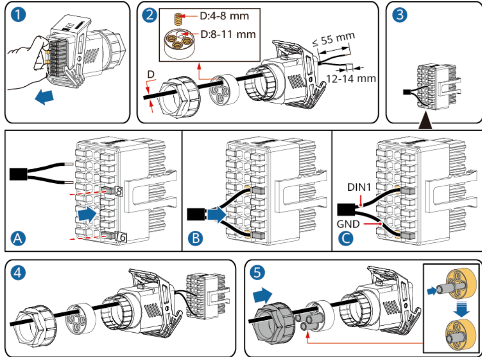
Figure 5-44 Installation du câble
