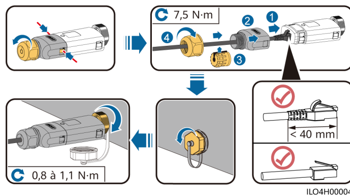
Figure 5-16 Installation du Smart Dongle WLAN-FE (communication FE)
