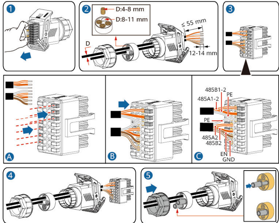
Figure 5-36 Installation des câbles
