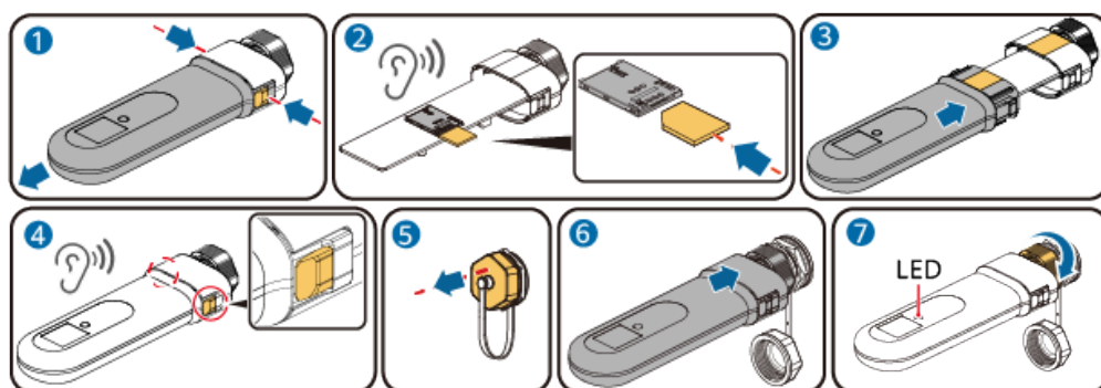
Figure 5-18 Installation du Smart Dongle 4G (SDongleB-06)
