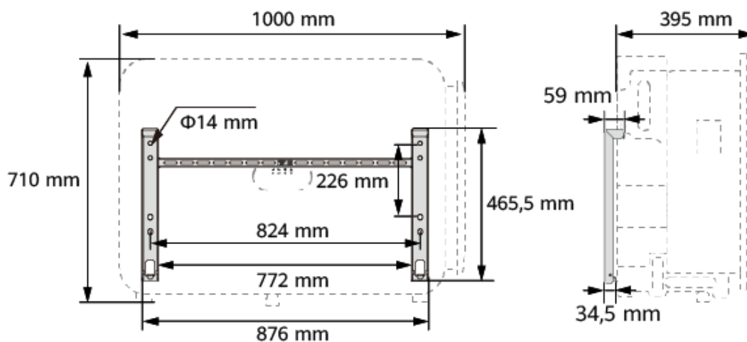
Figure 4-1 Dimensions
