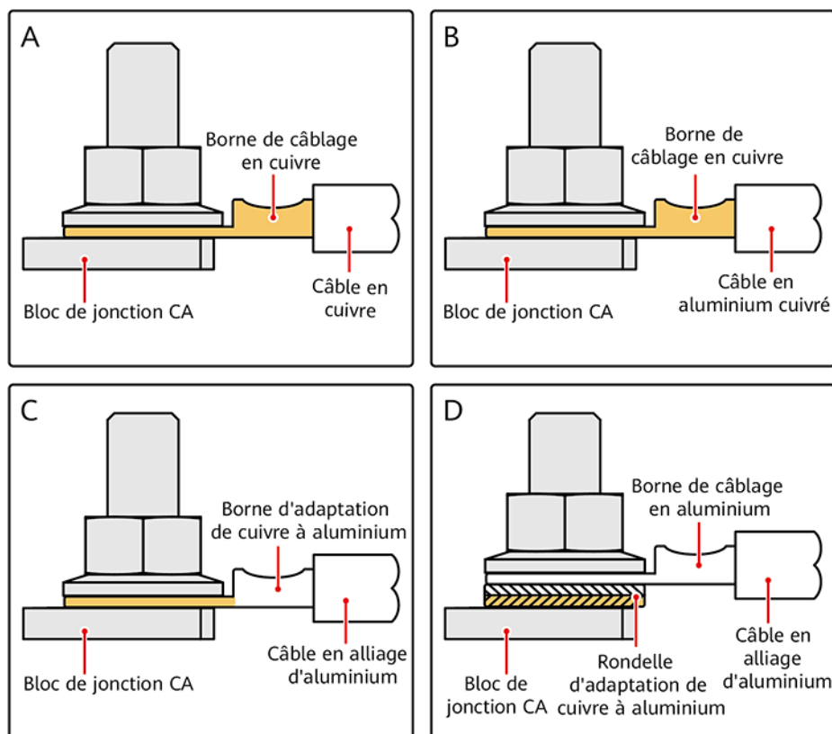
Figure E-1 Exigences relatives à la borne OT/DT
