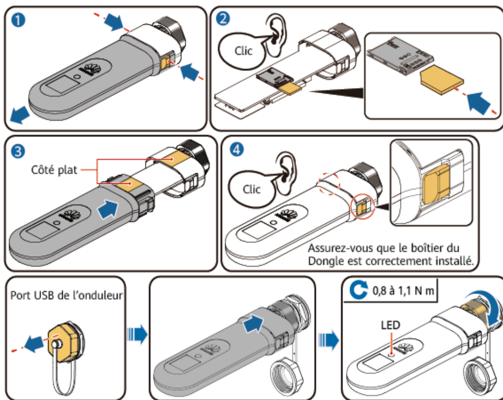
Figure 5-19 Installation du Smart Dongle 4G (SDongleB-06)
