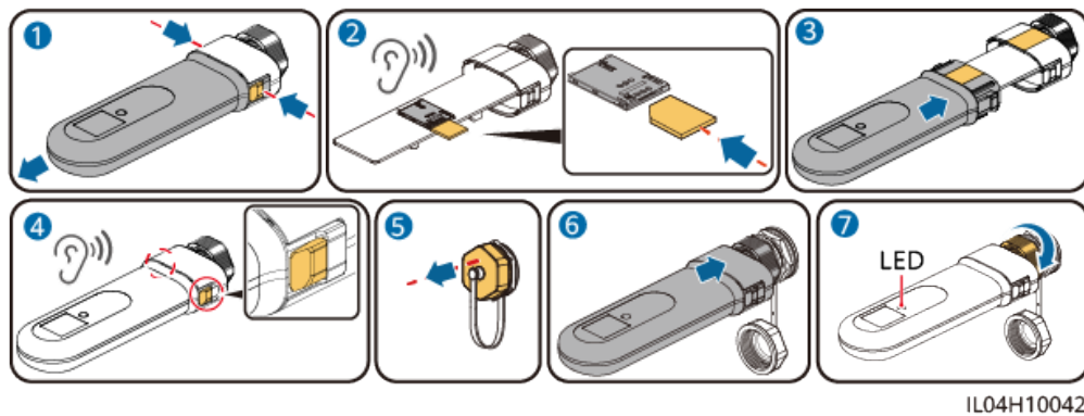
Figure 5-47 Installation du Smart Dongle 4G (SDongleB-06)
