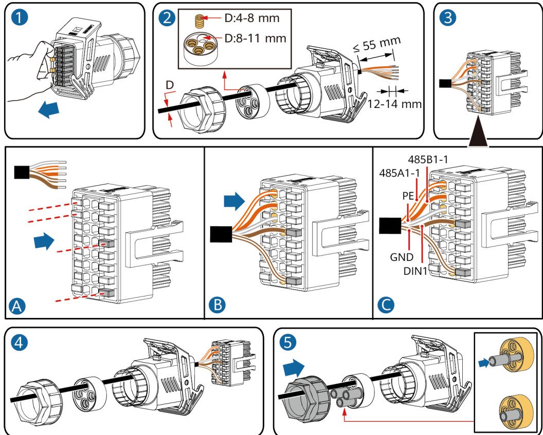
Figure 5-34 Installation du câble
