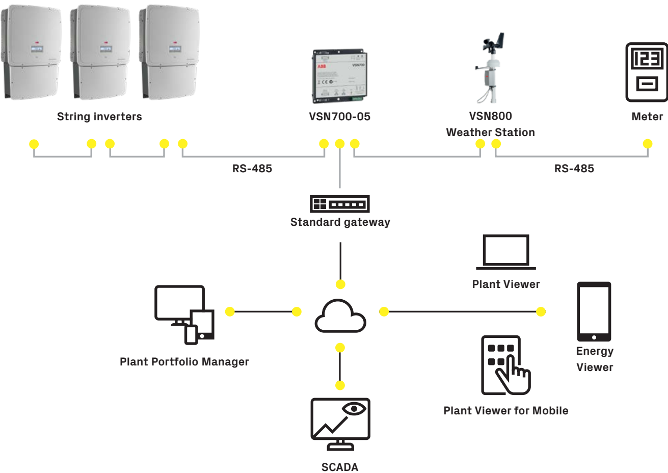
Application with TRIO and PVI string inverters
