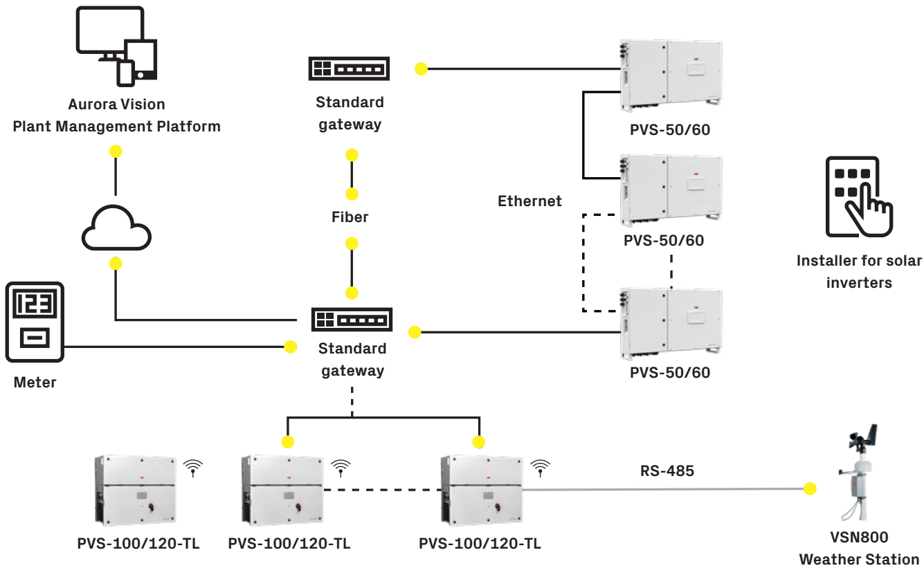
Application with PVS string inverters
