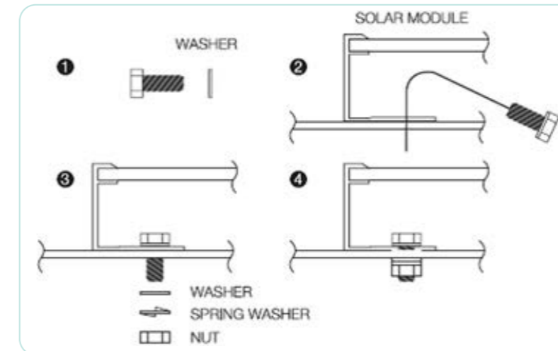
Figure 3. Mounting using bolts on the transversal bars.
