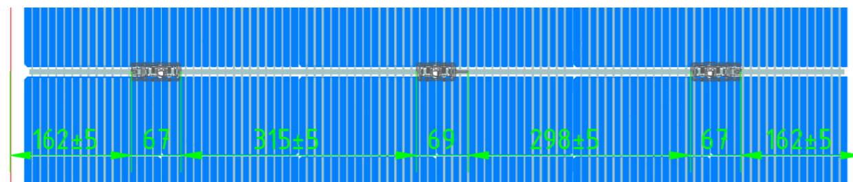
Figure 6. Position of the junction box of frameless module
